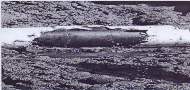
picture showing two (2) cuts on the pipeline.
